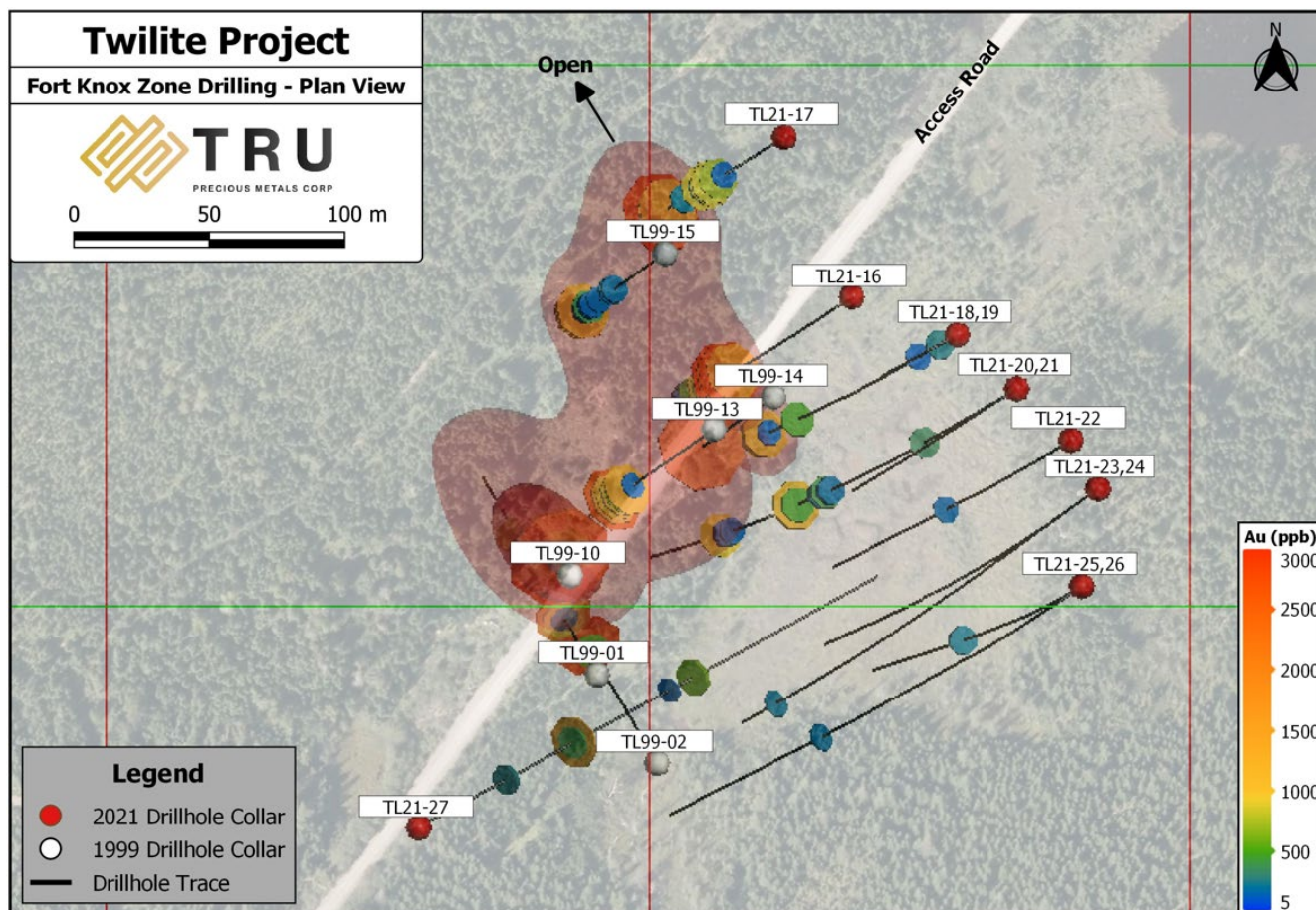
Figure 1. Plan Map of Twilite Gold Drilling
