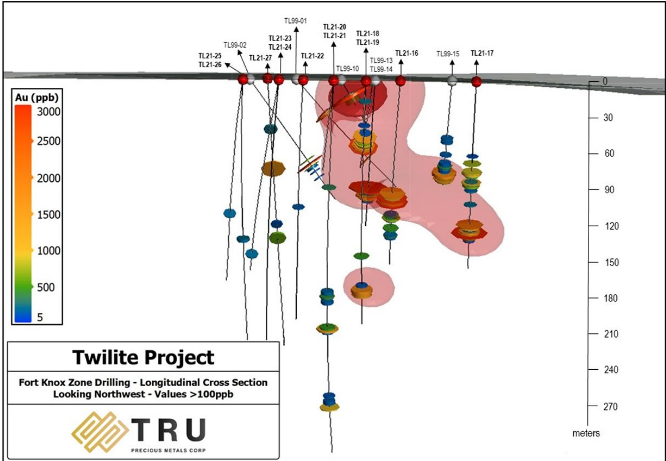
Figure 2. Longitudinal Cross Section of Fort Knox Gold Zone
